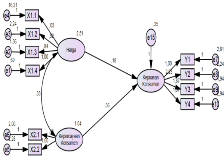
Gambar 1 Model Struktural
