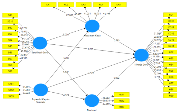
Figure 2. Inner Model Measurement Results
